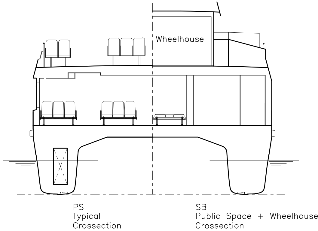
Crosssection
